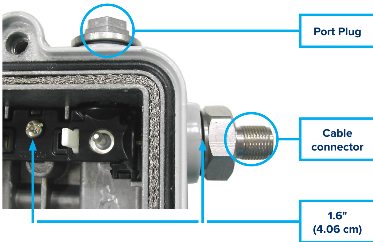
Figure 3: Cable connector
