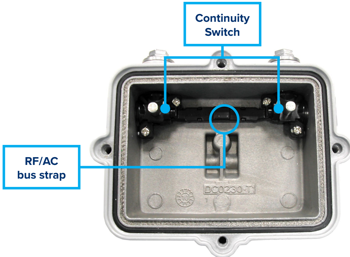
Figure 6: Internal view of OTRWXU housing base
