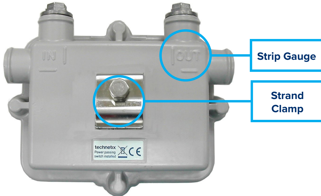
Figure 4: Housing base (OTRWX-X-XX shown)
