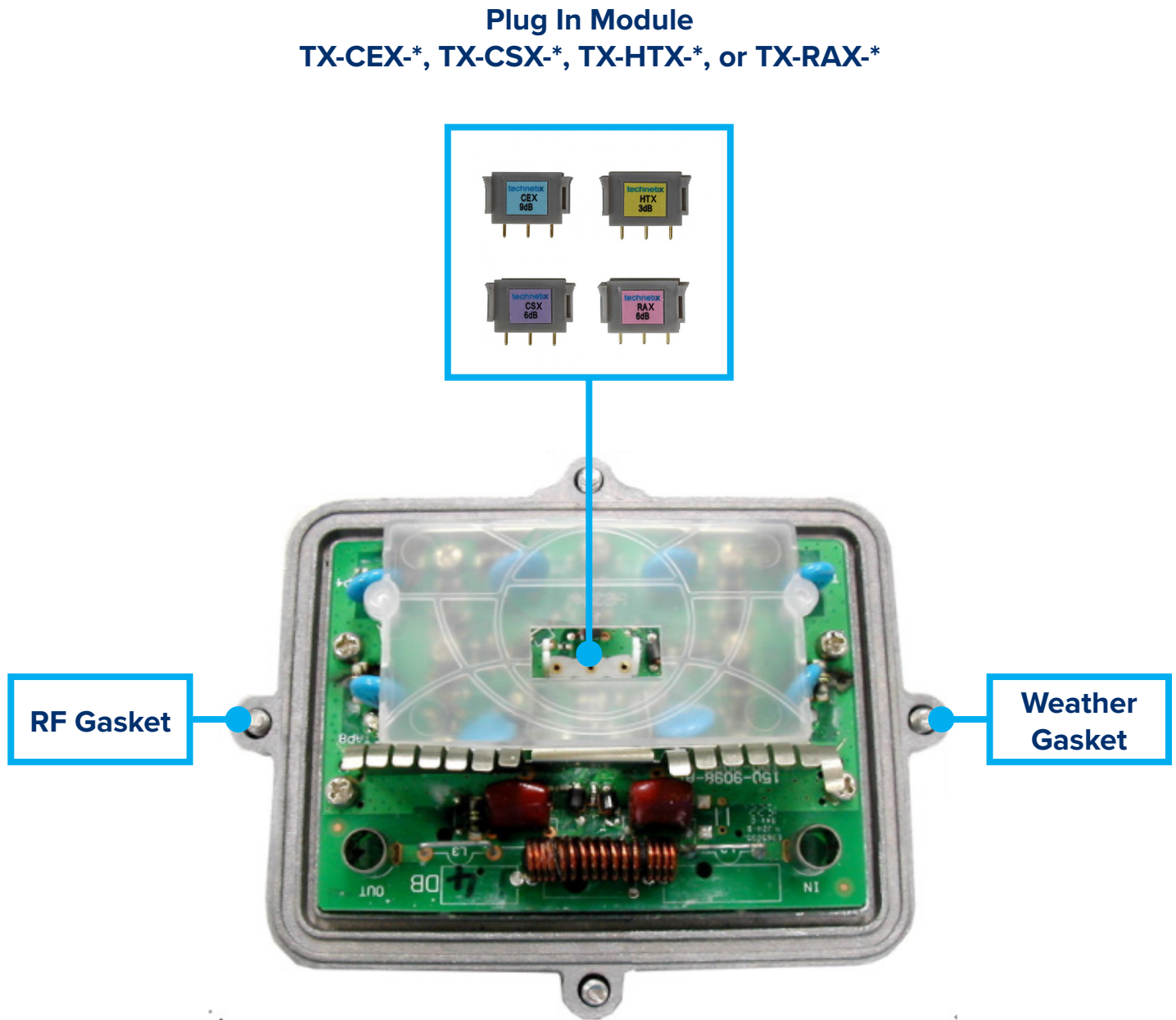
Figure 9: Plug-In modules
